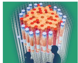
Neutronics and thermal-hydraulics Coupling for SMR
